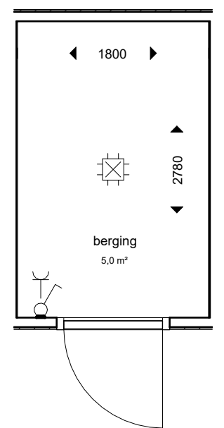
berging 1:50
