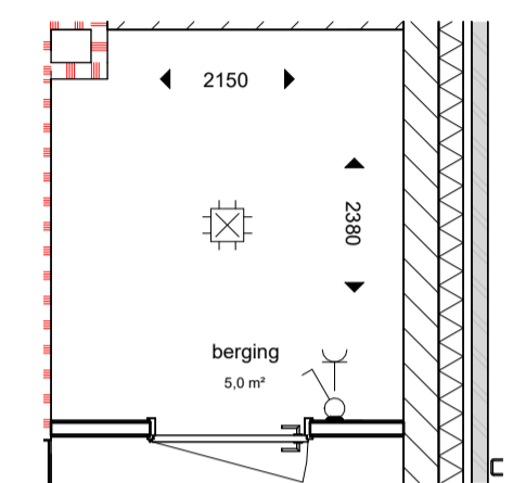
berging 1:50
